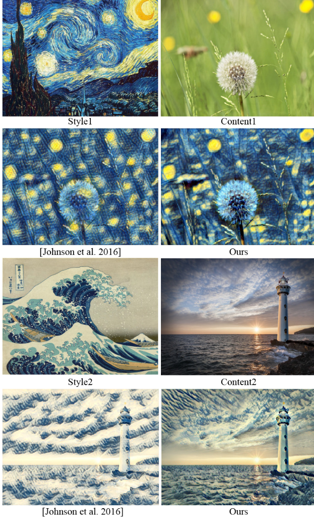
Figure 3: Qualitative result comparison with [Johnson et al. 2016]. We can see that the style of the original method tends to be distributed fairly evenly, which thus obscures the image layout. In contrast, our image stylization method better retains the structure of the content image. Content images are from Pixabay. Style1: The Starry Night by Vincent van Gogh. Style2: The Great Wave by Hokusai.
